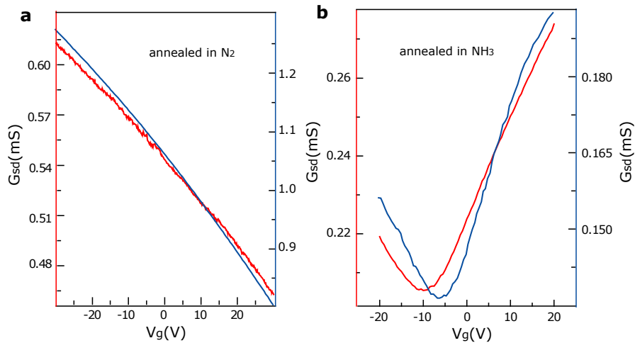
Figure S2. The transport data measured in vacuum for different graphene-based FETs. The different color of the G_{sd} - V_g curves indicates different devices annealed in N_2 and in NH_3 . The graphene was annealed (a) in N_2 and (b) in NH_3 after irradiation, and the variation of data is due to the difference of the device fabrication.
